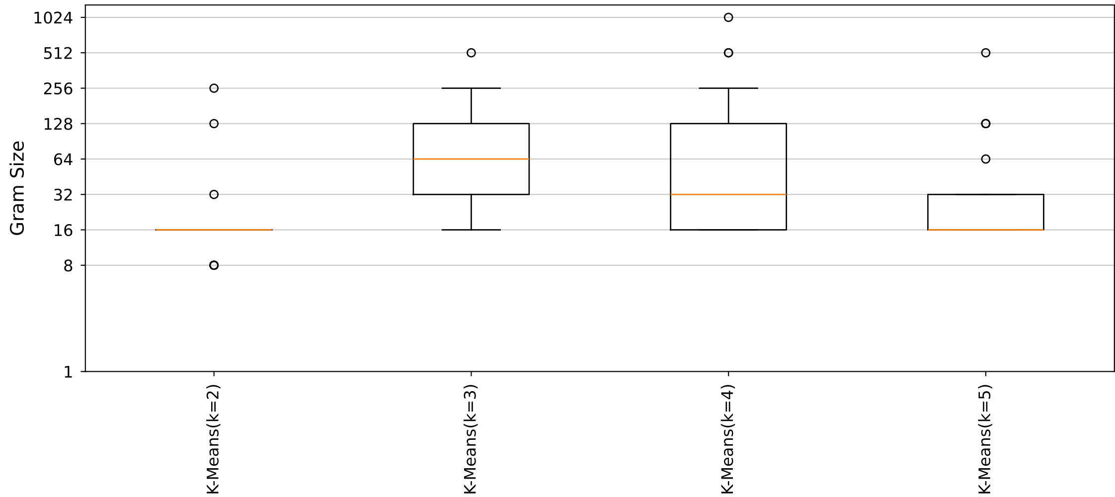
YARA Rules Gram Size Distribution (Cluster40_Size5 dataset)
